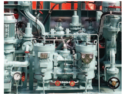
HFO Booster Module Diesel Engine various Shipyard STX DACT Filter - Filtration 35 µm absolute
