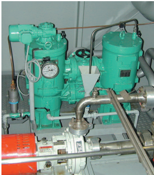
Booster System - Gas Turbine GE LM 2500 Ship "JEWEL OF THE SEAS" DACXT Filter - Filtration 10 µm absolute
